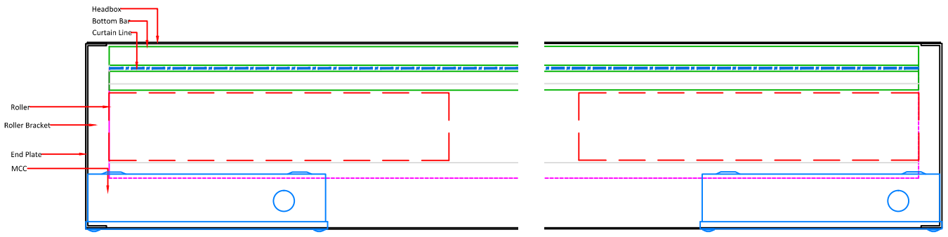
03 001 Plan Section Of Through Headbox SCALE 1:5 @ A3
