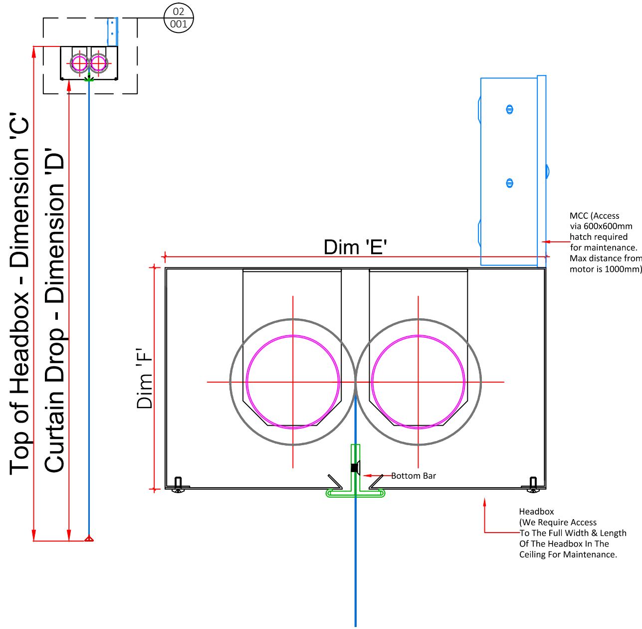
02 Section Through Headbox SCALE 1:3 @ A3
