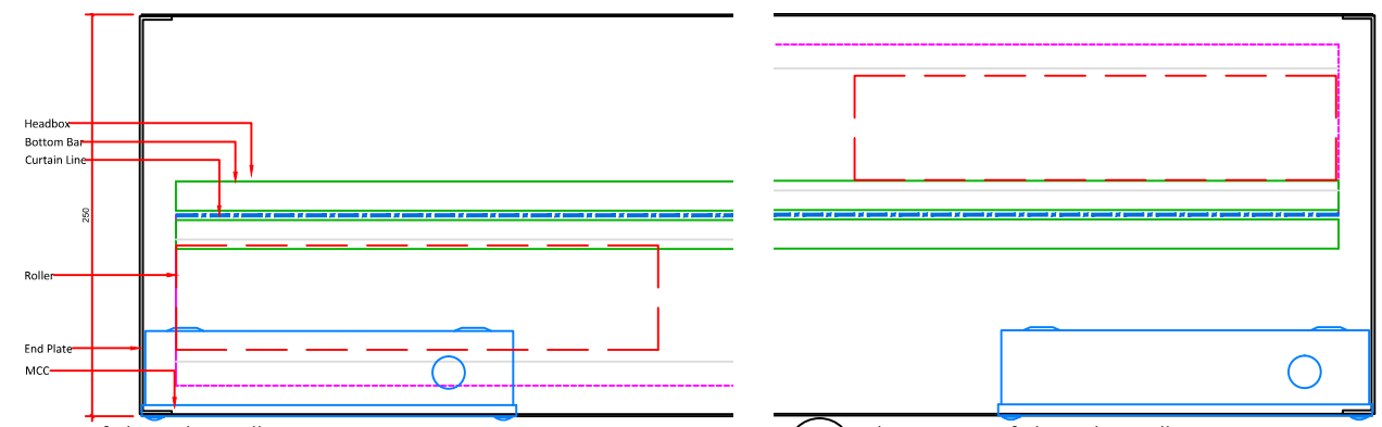
03 Plan Section Of Through Headbox SCALE 1:5 @ A3
