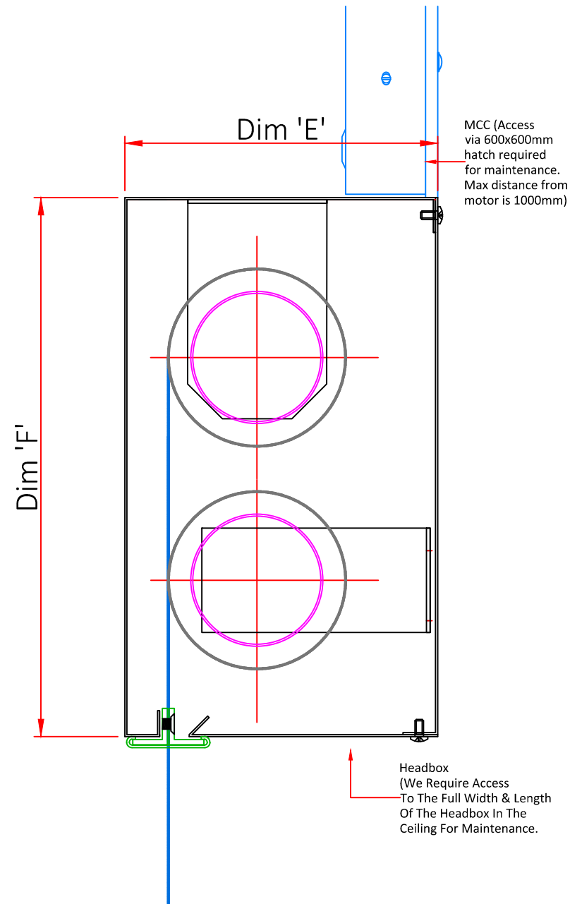
02 Section Through Headbox 001 SCALE 1:3 @ A3
