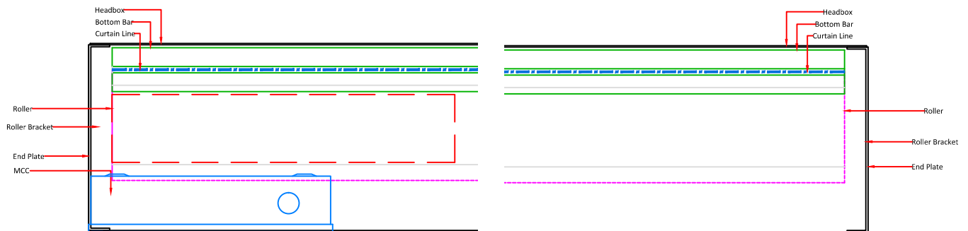
03 Plan Section Of Through Headbox 001 SCALE 1:5 @ A3
